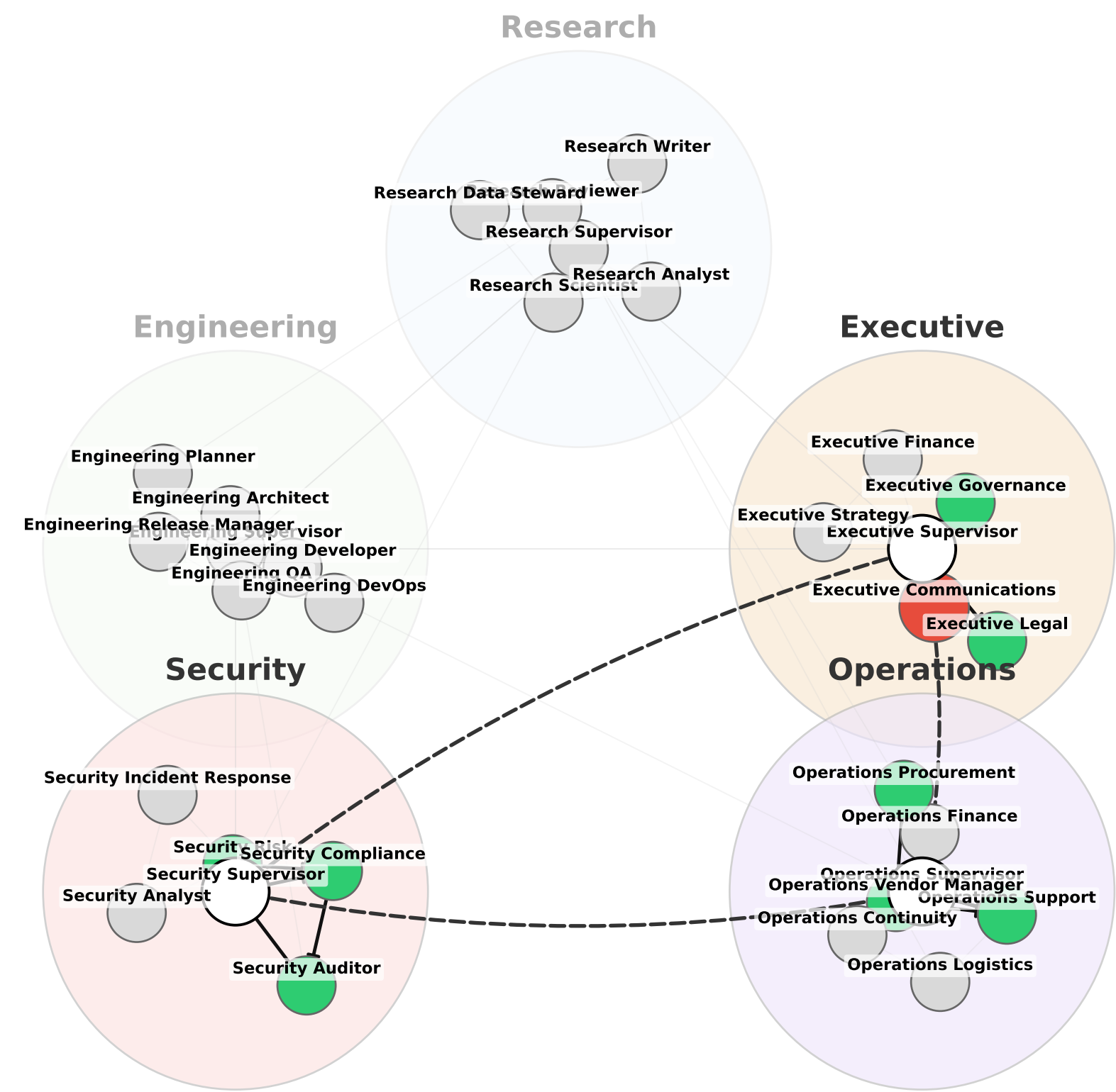
(a) Runtime Trust Graph
